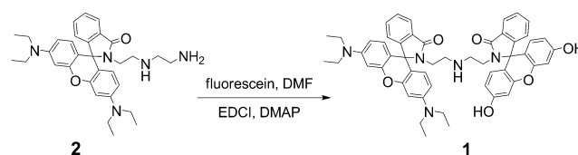
Scheme 1. Synthetic route to 1 . DMF = N,N -dimethylformamide, EDCI = 1-ethyl-3-(3-dimethylaminopropyl)carbodiimide, DMAP = 4-(dimethylamino)pyridine.
